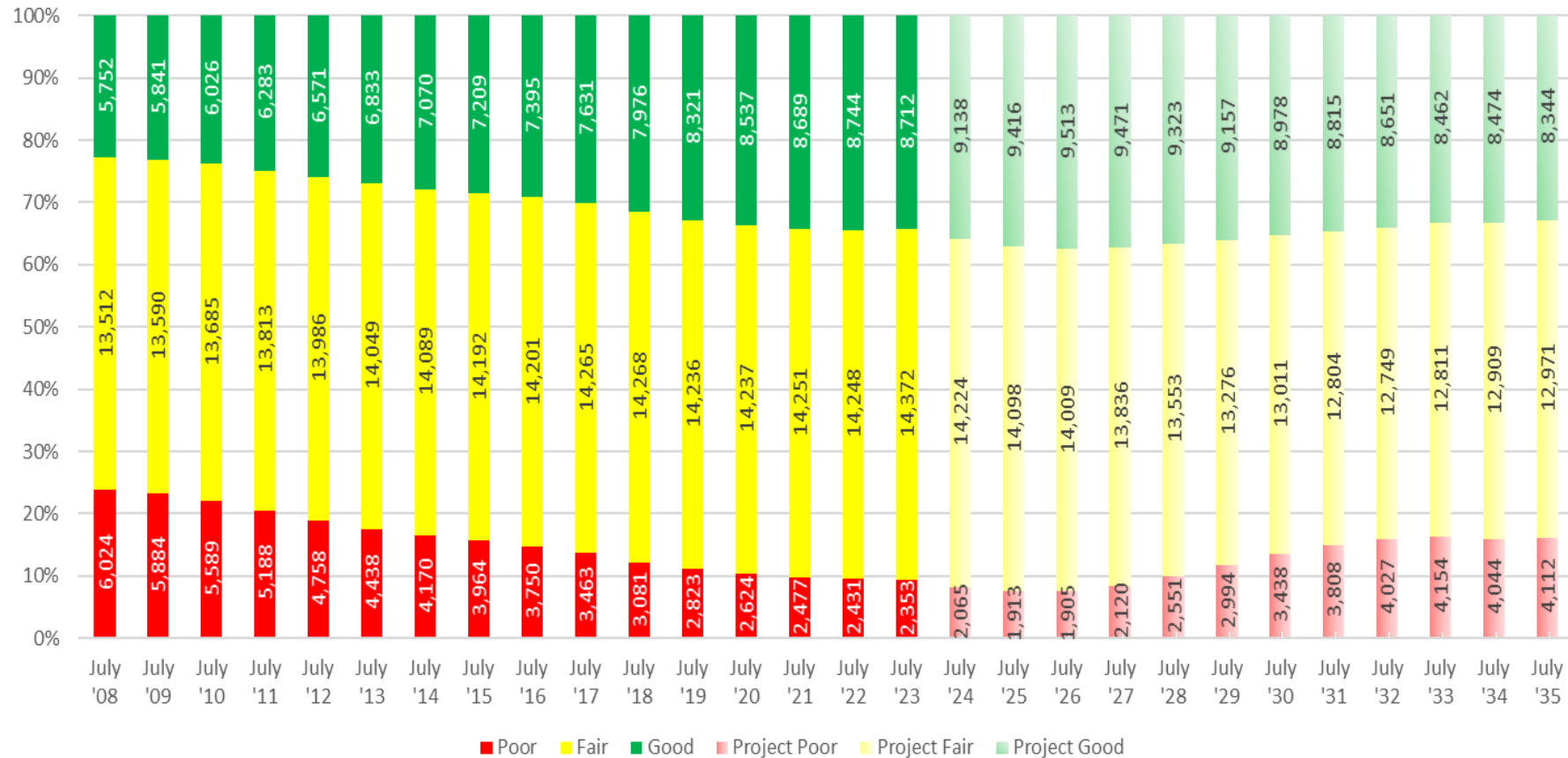
State Owned - Bridge Condition 2008 - 2023 Actual 2024 - 2035 Projected with Additional 600M Funding (Bridge Count)
